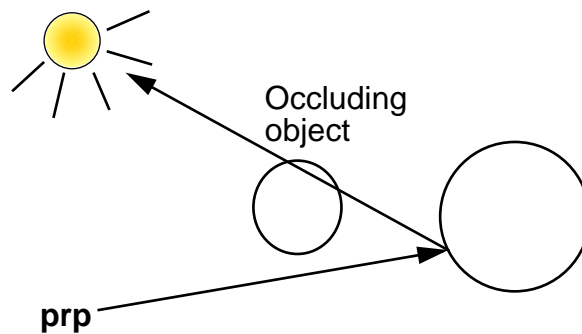
FIGURE 212. The shadow ray tests whether or not a surface point is visible from the light source or not
