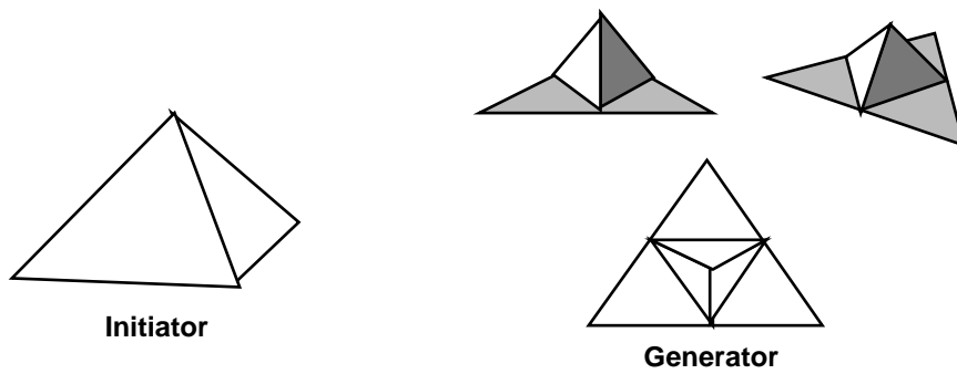
FIGURE 86. Self-similar fractals in 3D
