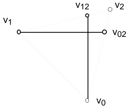
FIGURE 196. dx and dy can be calculated by interpolating the intermediate points v02 and v12 and their intensity values.
