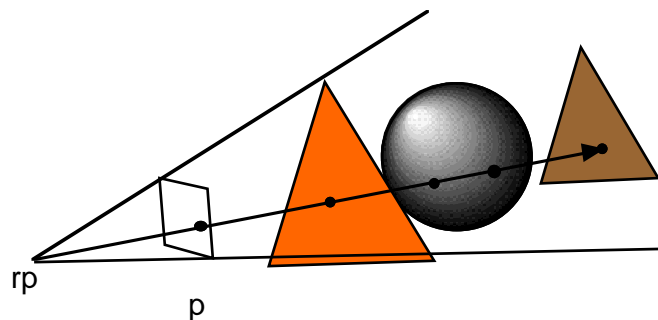
FIGURE 208. Ray-casting in a scene. A ray is formed through prp and a pixel in the image plane.
