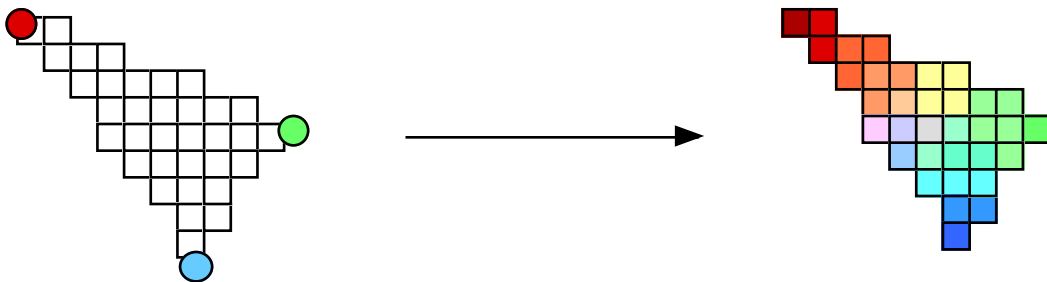
FIGURE 41. The fragment processor generates colors for each fragment
