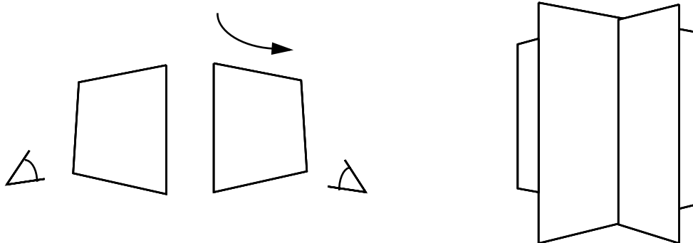
FIGURE 142. A billboard (left) is a single polygon always facing the viewer. Two or three polygons, with no rotation to face the viewer (right) gives higher realism
