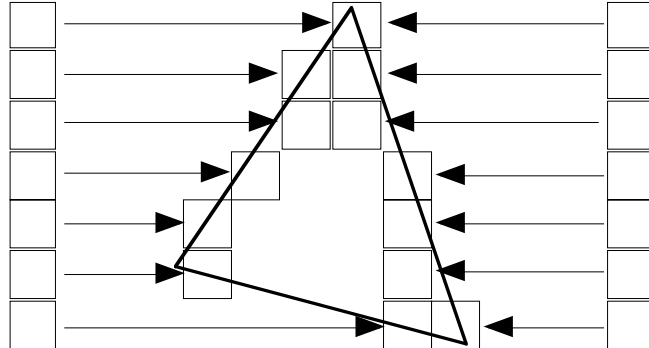
FIGURE 195. Filling the span buffer
