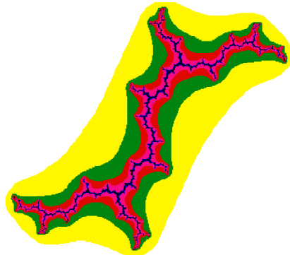
FIGURE 93. Julia set for L = (0, 1) = 0 + j
