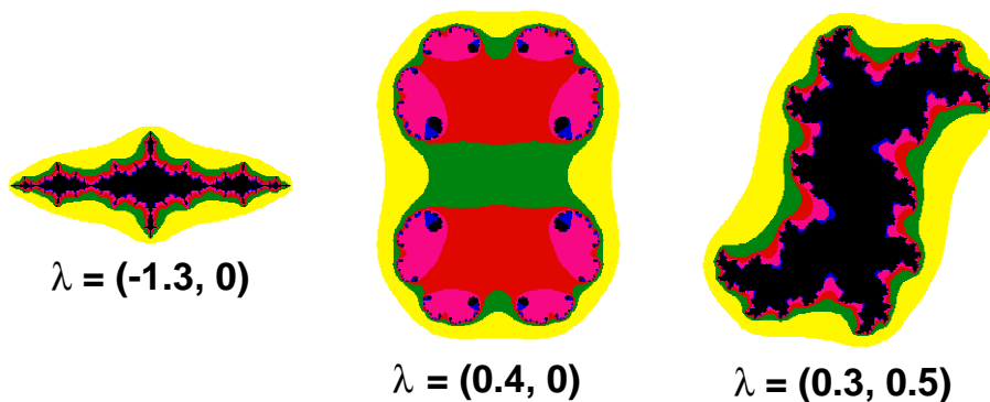
FIGURE 94. Other Julia sets
