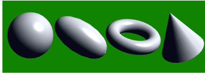
FIGURE 65. Quadrics: sphere, ellipsoid, torus, cone
