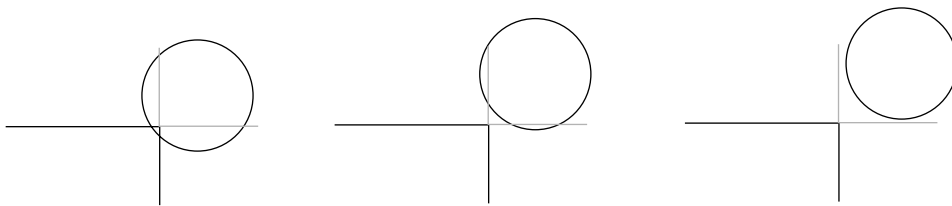
FIGURE 164. Sphere-corner test using planes only. Left: Correct hit. Middle: False hit. Right: Correct miss.
