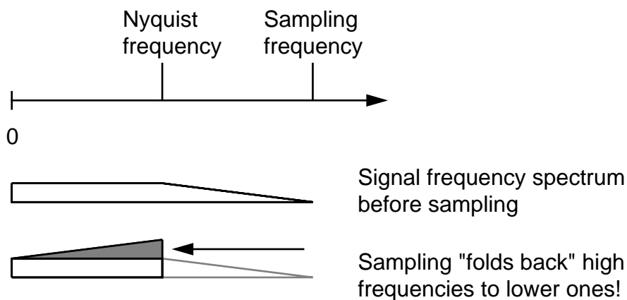
FIGURE 202. Higher frequencies are “folded” over the Nyquist frequency
