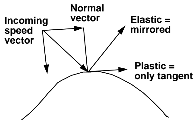
FIGURE 173. Simple particle-surface collision handling
