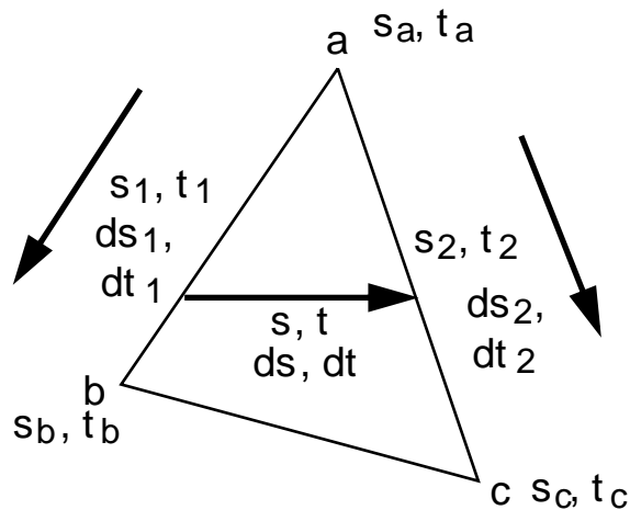
FIGURE 198. Affine texture mapping, linear interpolation
