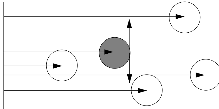
FIGURE 172. Collision detection accelerated by linear sorting
