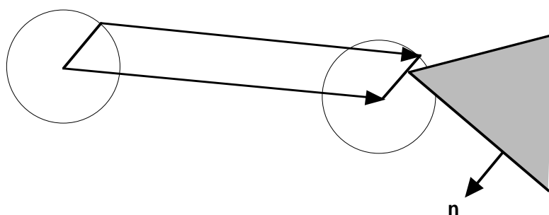
FIGURE 171. A case where the speed vector doesn't intersect any polygon, but we should still detect a collision!
