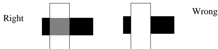
FIGURE 133. A dark object behind a semi-transparent white object, with a result depending on drawing order
