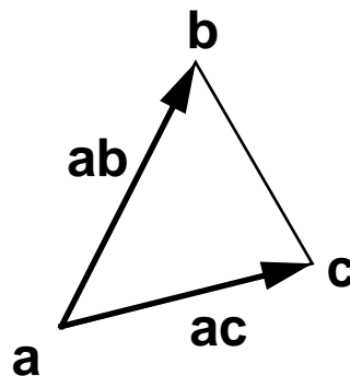
FIGURE 127. Screen space back-face culling – using a polygon projected to screen
