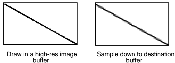
FIGURE 204. A line drawn without anti-aliasing and with super-sampling
