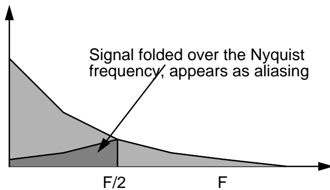
FIGURE 205. Aliasing without super-sampling
