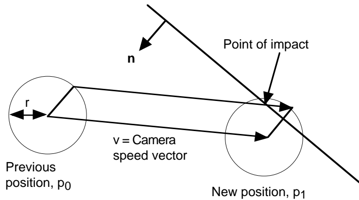
FIGURE 170. Collision camera to (infinite) plane
