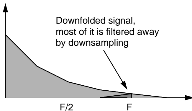
FIGURE 206. Super-sampling significantly reduces aliasing
