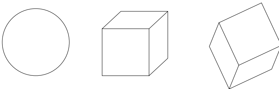
FIGURE 165. The three basic shapes for collision detection: sphere, AABB and OBB
