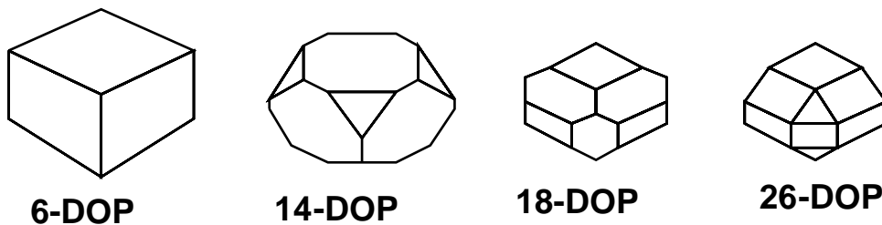
FIGURE 167. The four possible kinds of k-DOPs
