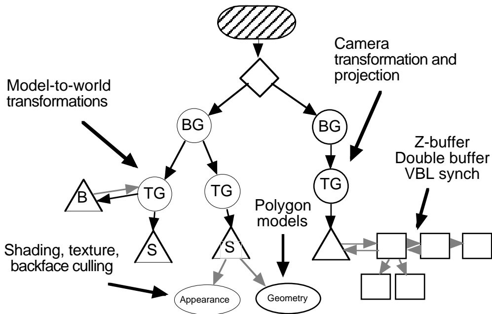
FIGURE 154. A Java 3D scene graph.
