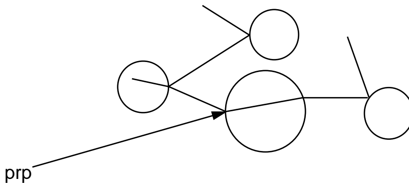
FIGURE 210. A ray is reflected and refracted in mirroring and transparent objects
