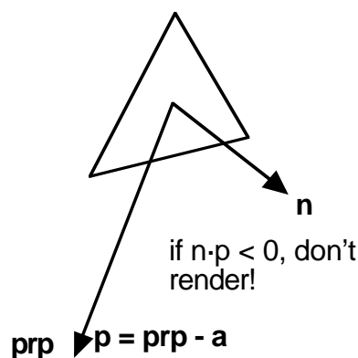
FIGURE 126. Camera space back-face culling
