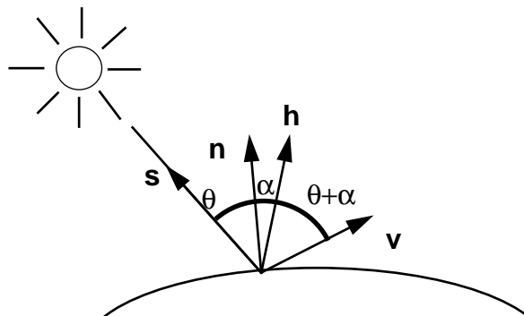
FIGURE 46. Specular reflection calculation using the halfway vector
