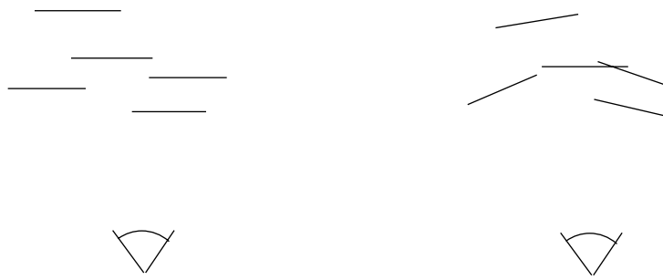
FIGURE 143. View plane (left) and viewpoint (right) oriented billboards.
