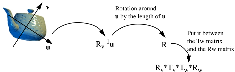
FIGURE 38. A way to implement trackball-style rotation from a mouse movement by \mathbf{v} .
