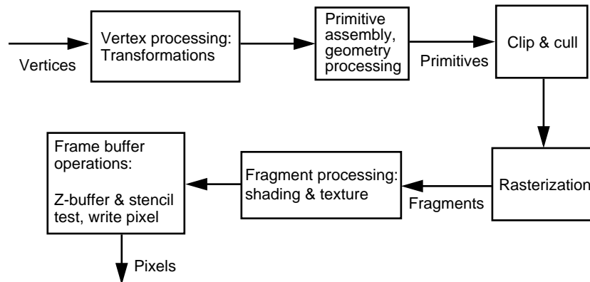
FIGURE 39. The OpenGL pipeline (simplified)
