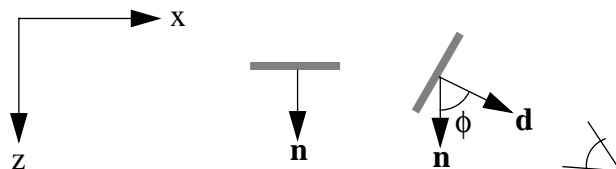
FIGURE 144. Axial billboard example, before rotation (middle) and after (right): The billboard is defined with its normal vector \mathbf{n} looking along Z, viewer in the \mathbf{d} direction.
