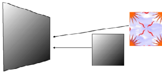
FIGURE 113. Light mapping with light map textures should be applied with multi-texturing
