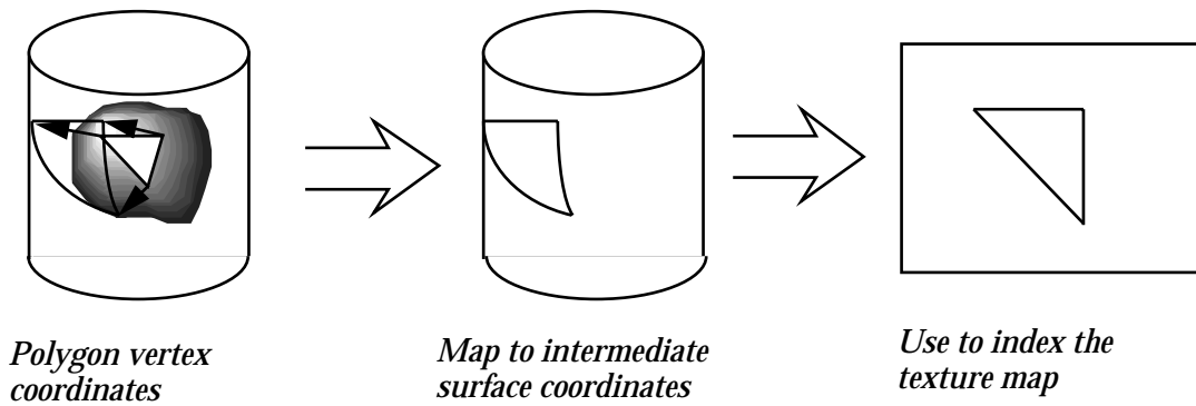
FIGURE 101. Texture coordinate generation
