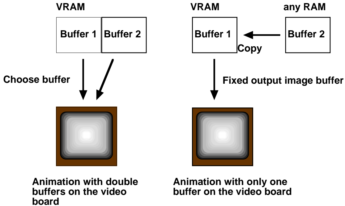
FIGURE 155. Two different cases of double buffering
