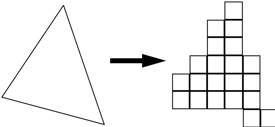
FIGURE 192. Scan conversion: From polygon to fragment (pixel) coordinates
