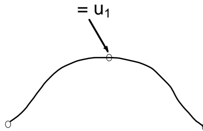
FIGURE 68. Two splines connected in a point
