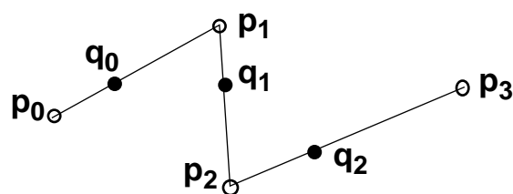
FIGURE 73. The four control points are blended to the spline by the blending functions
