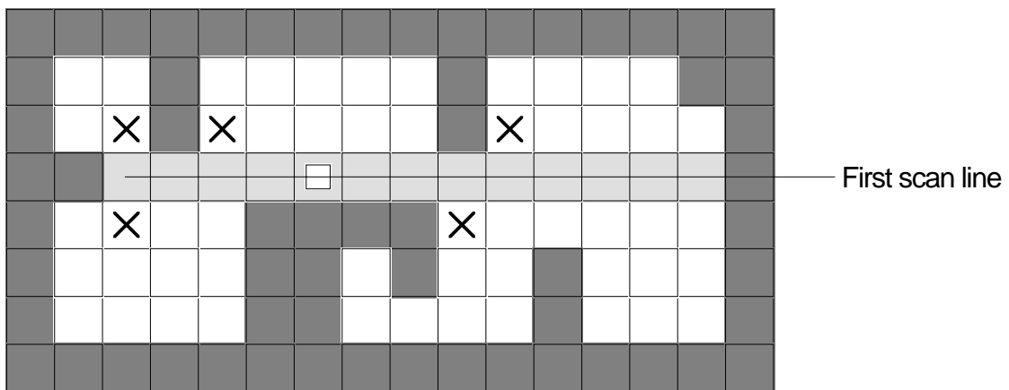
FIGURE 191. Flood fill
