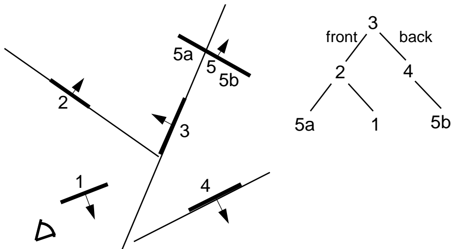
FIGURE 132. BSP tree example (Adapted from Foley, van Dam [27].)
