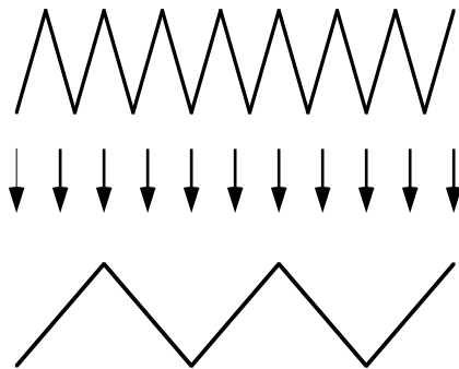
FIGURE 201. Example of how sampling can result in a lower frequency
