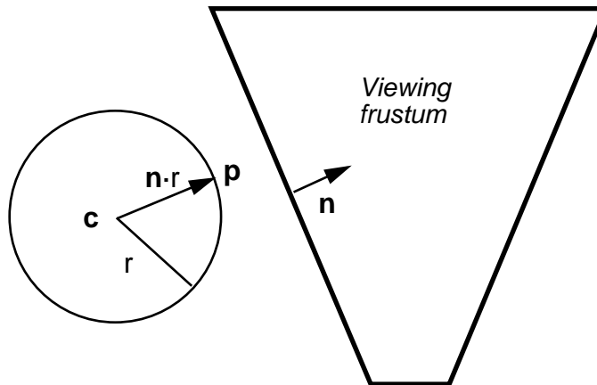
FIGURE 135. Sphere-frustum test used for bounding spheres of objects
