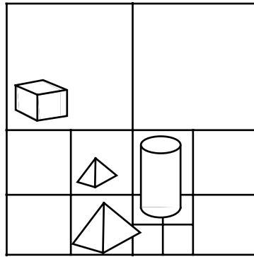
FIGURE 213. Subdivision of space into a quadtree to simplify searches
