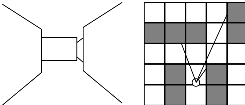
FIGURE 209. Ray casting in a 2D grid
