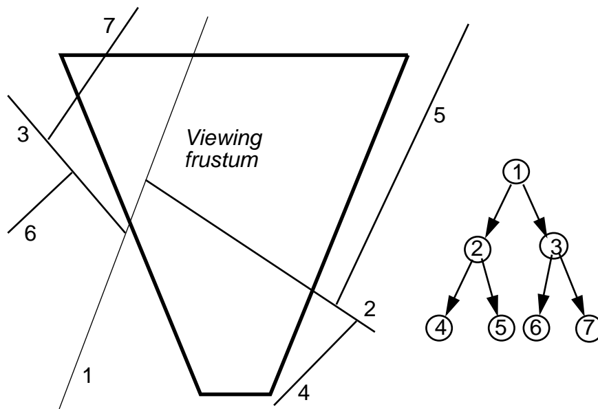
FIGURE 137. Clipping using a BSP tree
