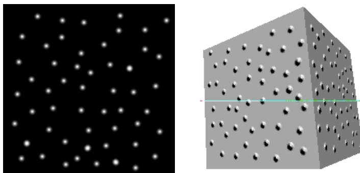
FIGURE 115. A bump map (left) applied to a cube (right)
