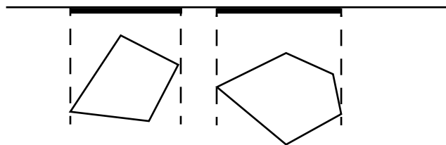
FIGURE 161. Two shapes projected onto an axis (top)
