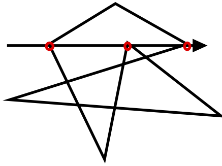
FIGURE 190. How do you count edges for a scan-line that passes through vertices?
