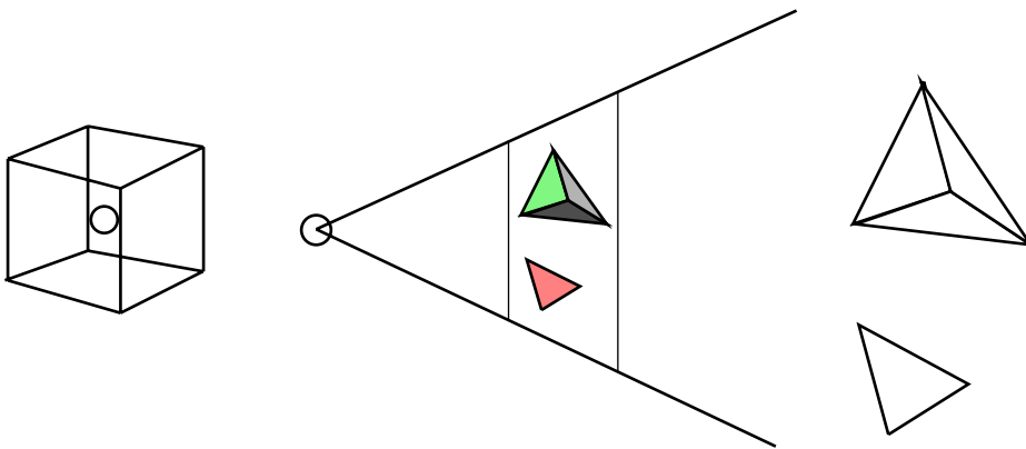
FIGURE 139. Image-space generation of PVS
