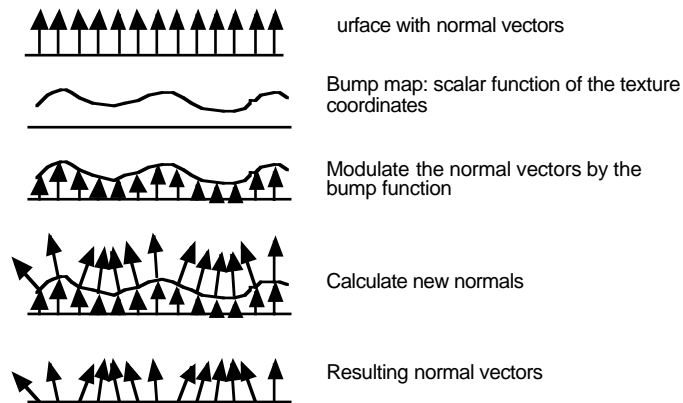
FIGURE 116. Principle for bump mapping
