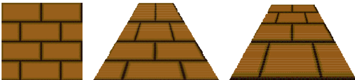
FIGURE 199. A texture, mapped on a polygon with affine and perspective correct mapping, respectively
