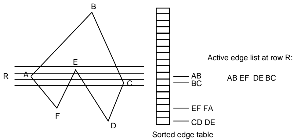
FIGURE 189. Scan-line polygon fill
