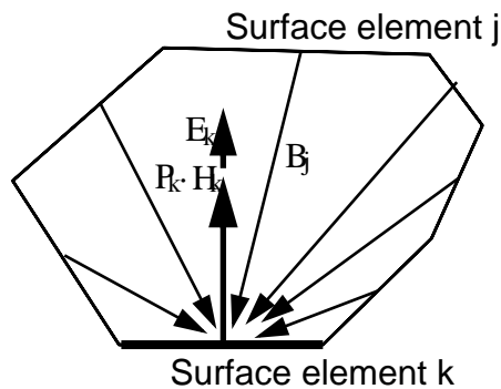
FIGURE 217. The light energy emitted from k is given by its own emission E_k and incoming light energy H_k
