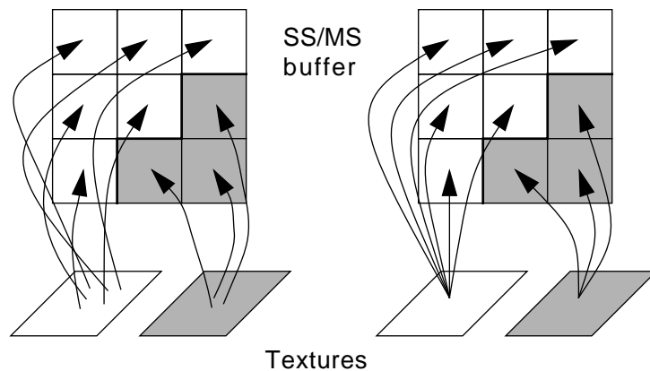
FIGURE 207. Comparison supersampling vs multisampling
