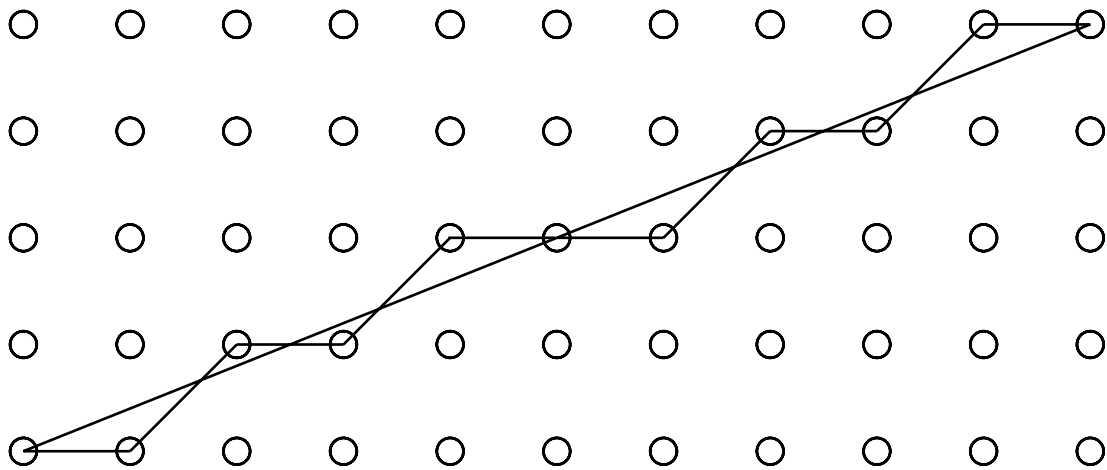
FIGURE 179. Example of line drawing with Bresenham's algorithm
