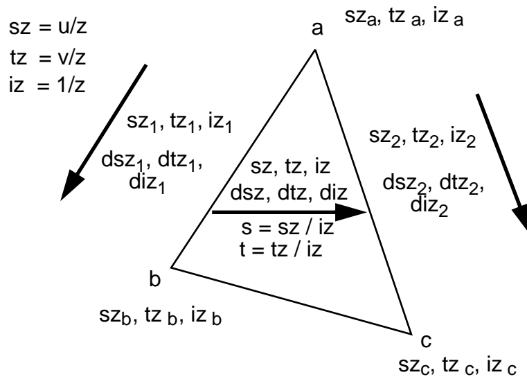
FIGURE 200. Implementation of perspective correct texture mapping
