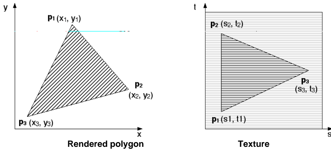
FIGURE 100. Texture mapping
