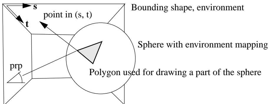
FIGURE 118. Environment mapping
