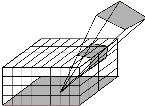
FIGURE 218. Enclosing half cube for approximation of form factors
