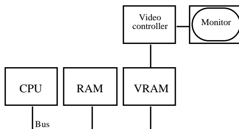
FIGURE 2. A graphics system with dedicated VRAM
