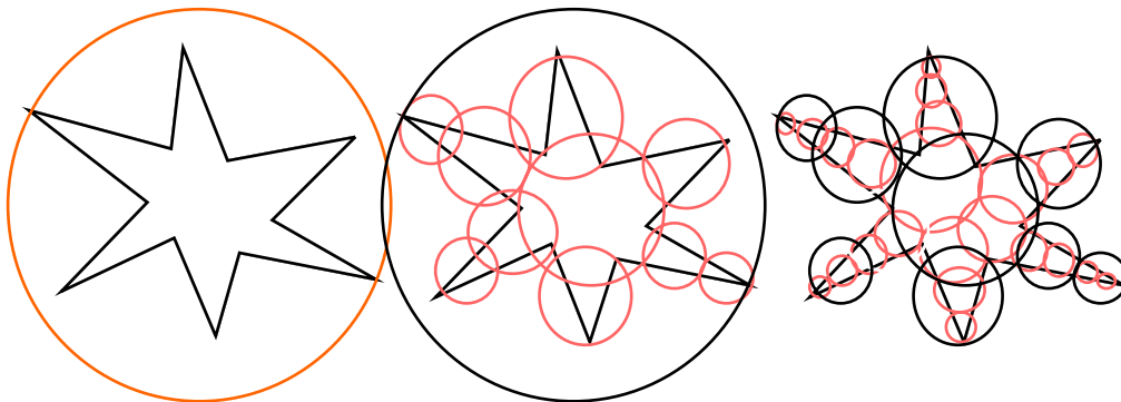
FIGURE 161. An example of a hierarchical collision detection system
