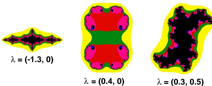
FIGURE 90. Other Julia sets
