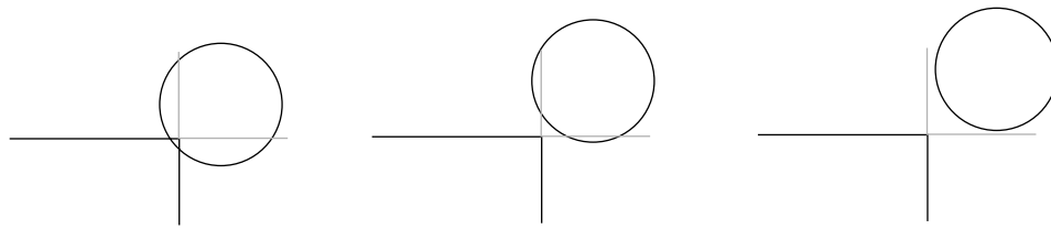
FIGURE 157. Sphere-corner test using planes only. Left: Correct hit. Middle: False hit. Right: Correct miss.
